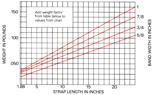
2300 SERIES STRAP WEIGHT GRAPH
